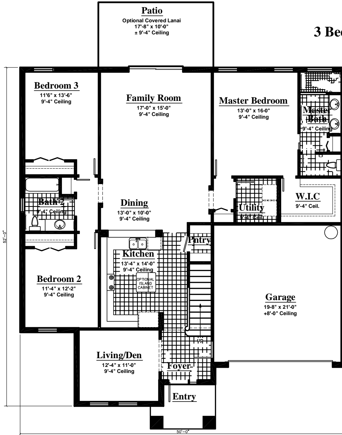
FIRST FLOOR
